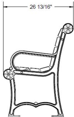
Overall Dimensions
