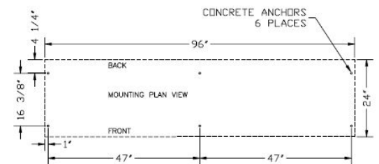
Diagram 5: Surface Mounting Instructions
