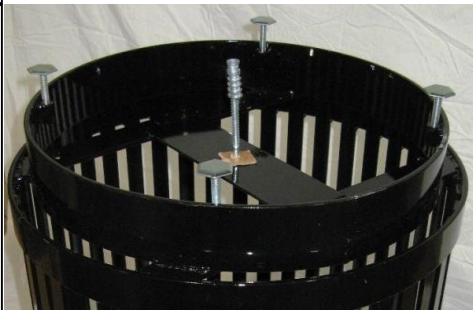
Bottom view Showing Leveling Feet and Anchor Bolt
